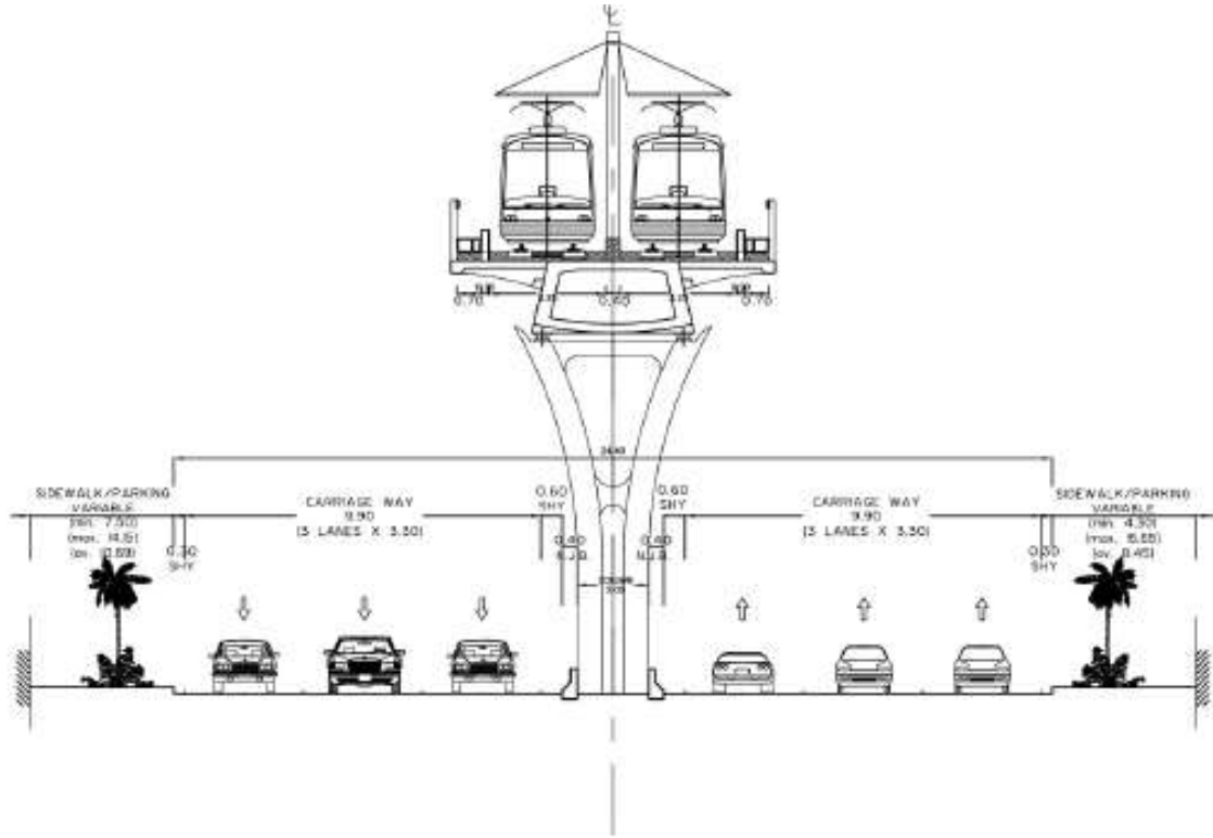
Figure 8.2: Typical Cross Sections of Mobility Corridors for Transit Systems
