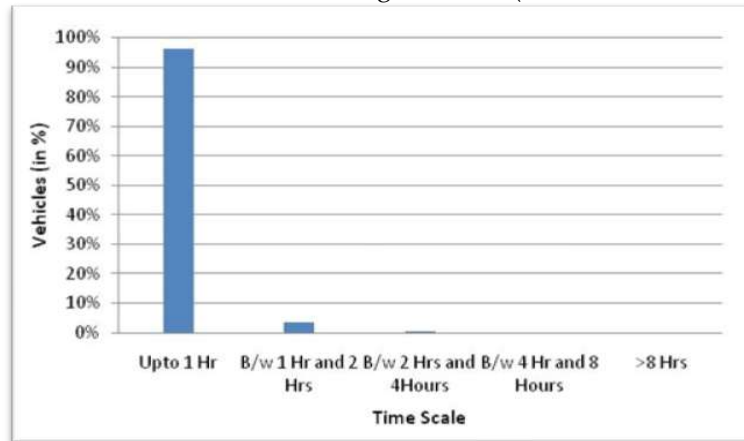
Figure 4.39: Classification of Parking Duration (Towards Wardha Road)
